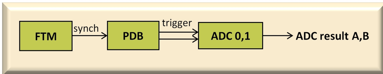
Figure 2. Peripheral interconnection
