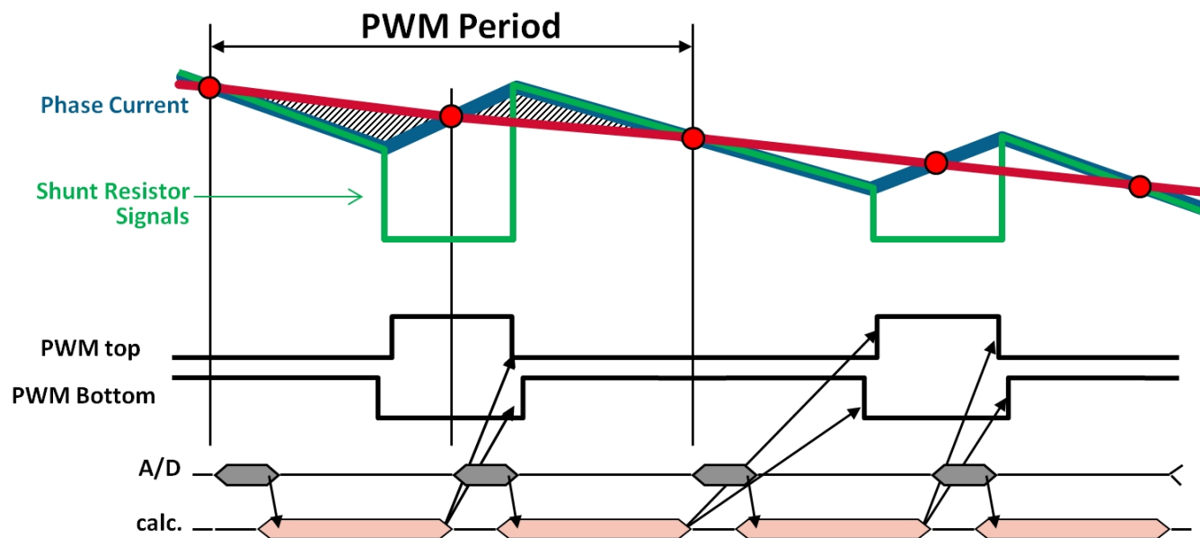
Figure 1. Synchronization principle
