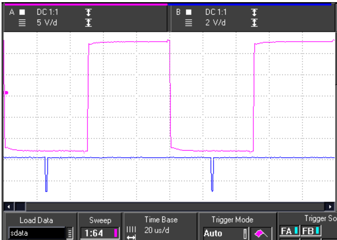
Figure 5. Measured waveforms: One pair per PWM.
