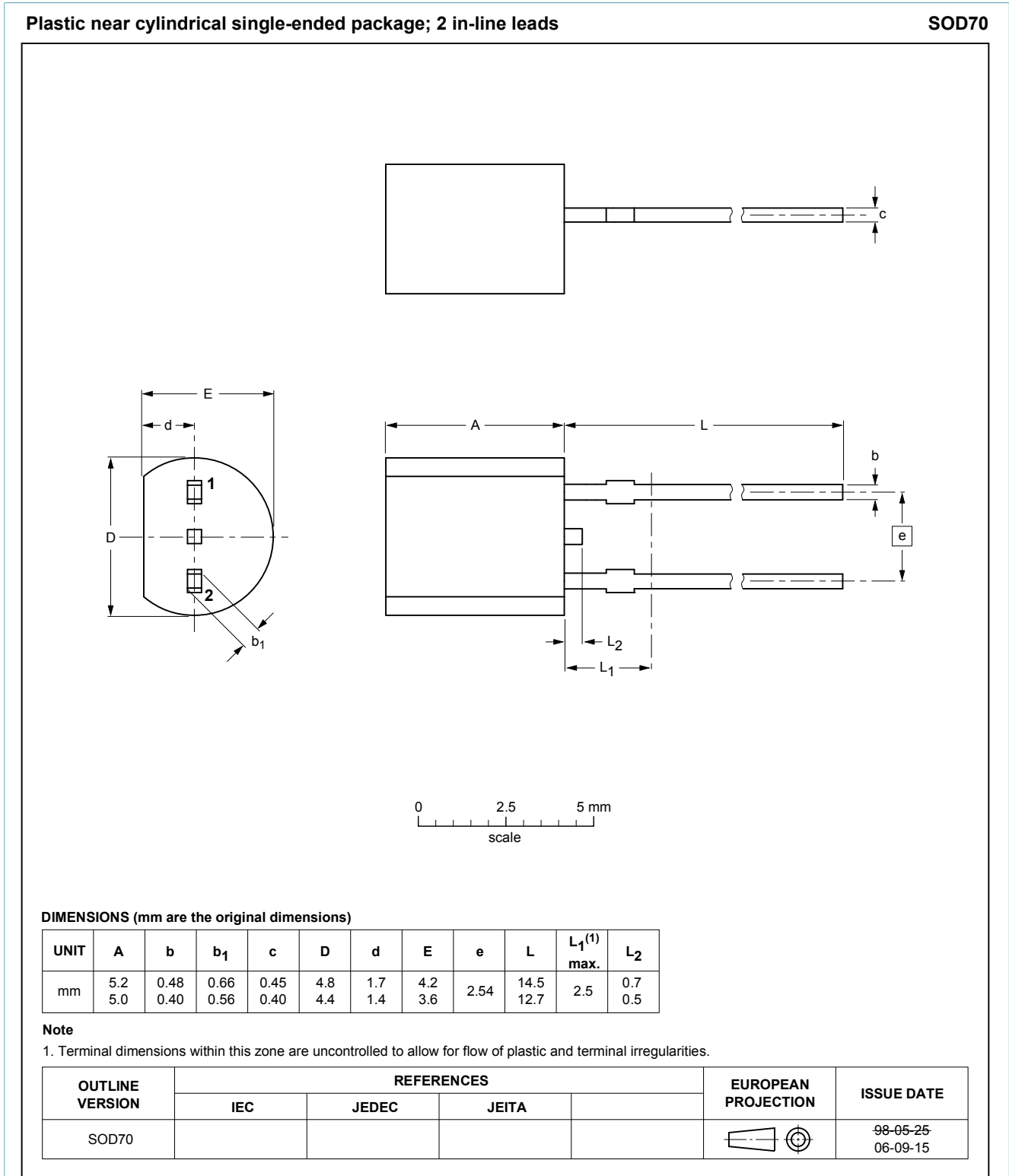
Fig. 1. Package outline PBCYT2 (SOD70)
