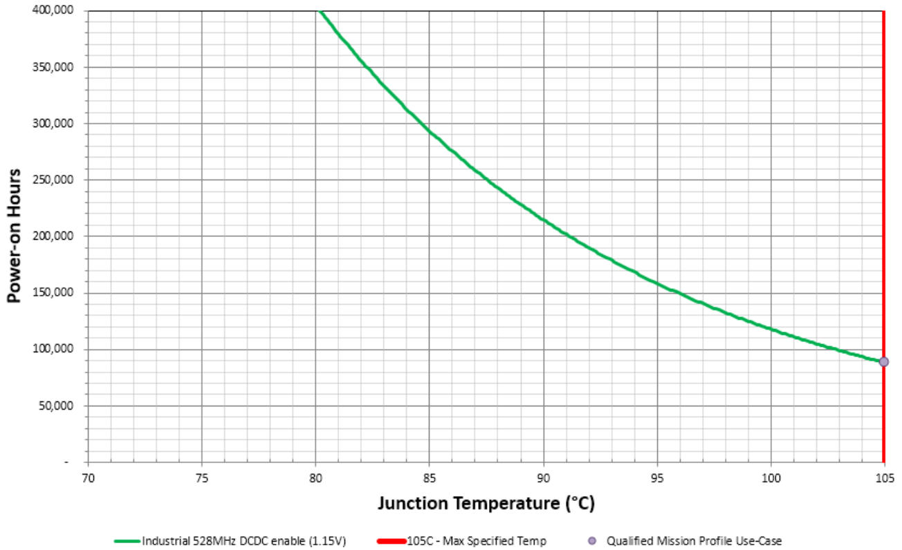
Figure 3. i.MXRT1050 Industrial lifetime estimates DCDC-enabled mode
