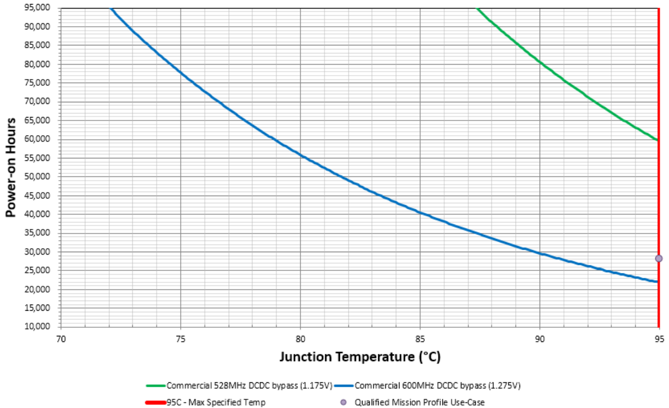
Figure 2. i.MXRT1050 commercial lifetime estimates, DCDC-bypass mode
