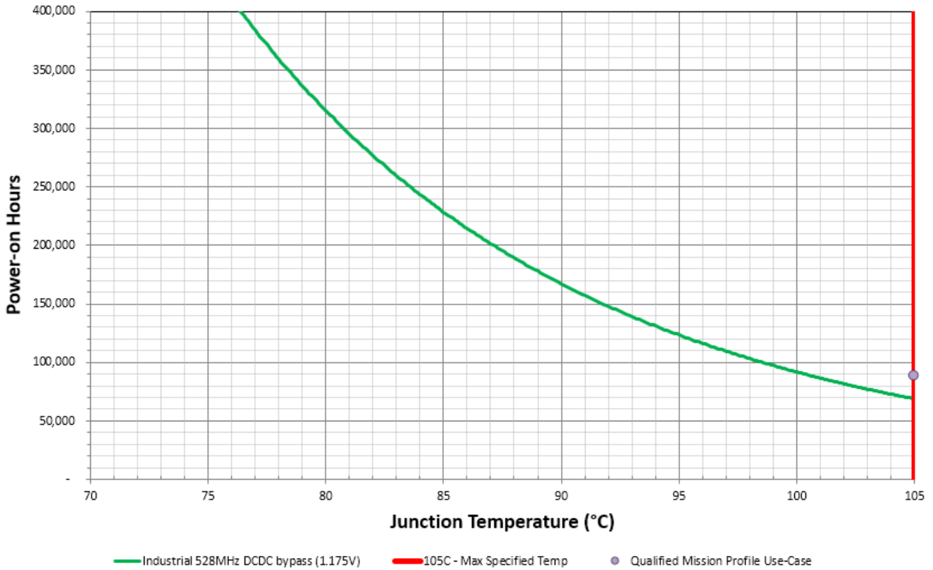
Figure 4. i.MXRT1050 Industrial lifetime estimates DCDC-bypass mode
