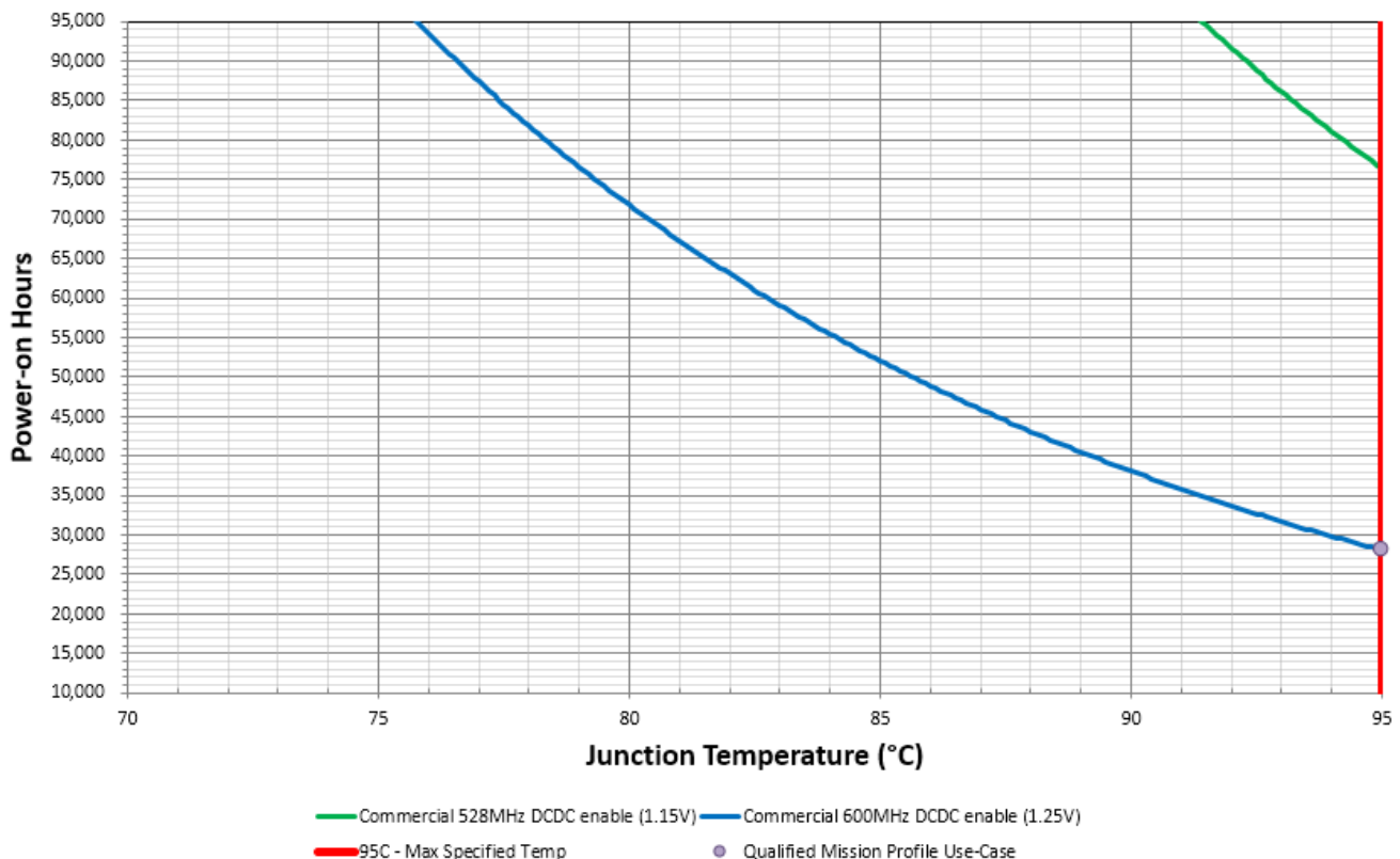
Figure 1. i.MXRT1050 commercial lifetime estimates, DCDC-enabled mode
